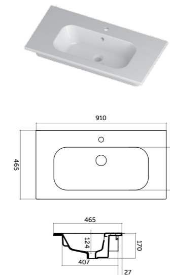
Consolle Qubo Square 121 - P 46 Console Qubo Square 121 - P 46
